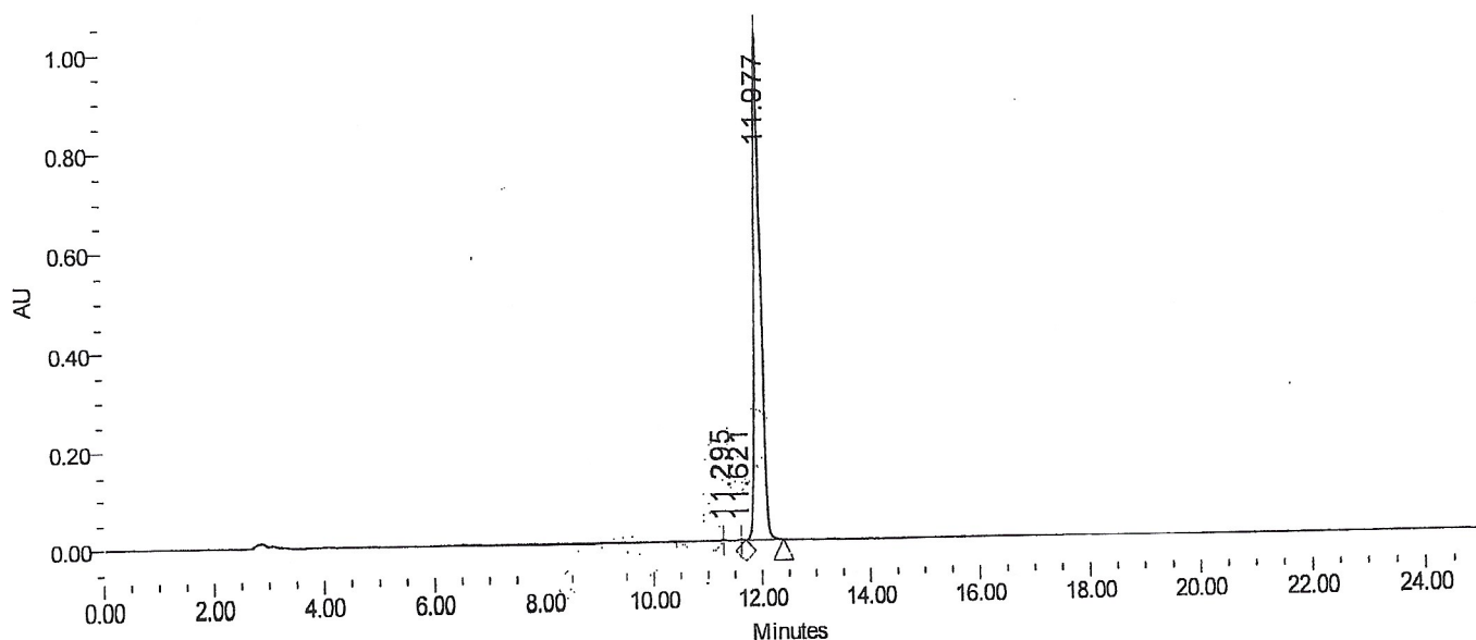
Auto-Scaled Chromatogram
